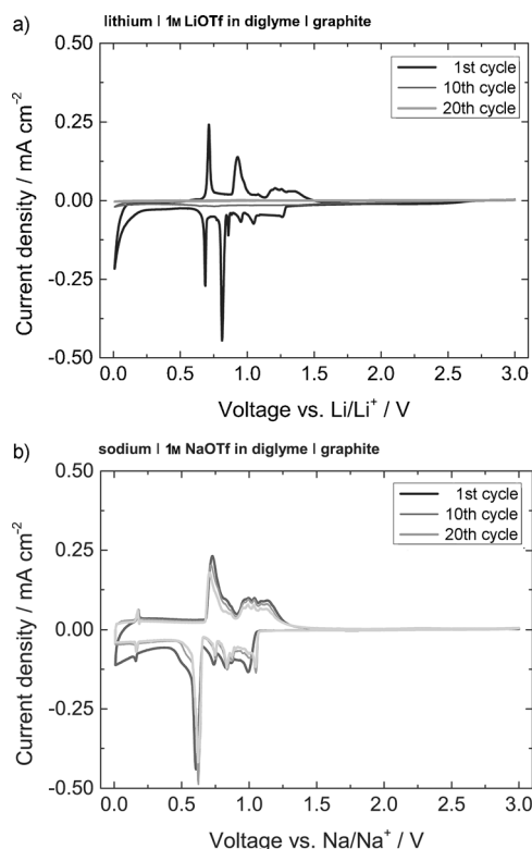
Figure 2. Redox behavior followed by cyclic voltammetry (sweep rate 0.05 \text{ mVs}^{-1} between 0.01 and 3.0 V).
